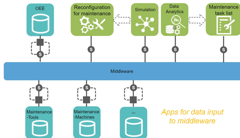
Fig. 2: Architecture Mapping for the Siemens Use Case.
