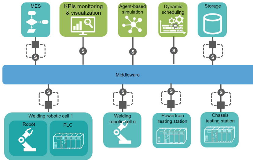
Fig. 3: Architecture Mapping for the IFEVs Use Case.
