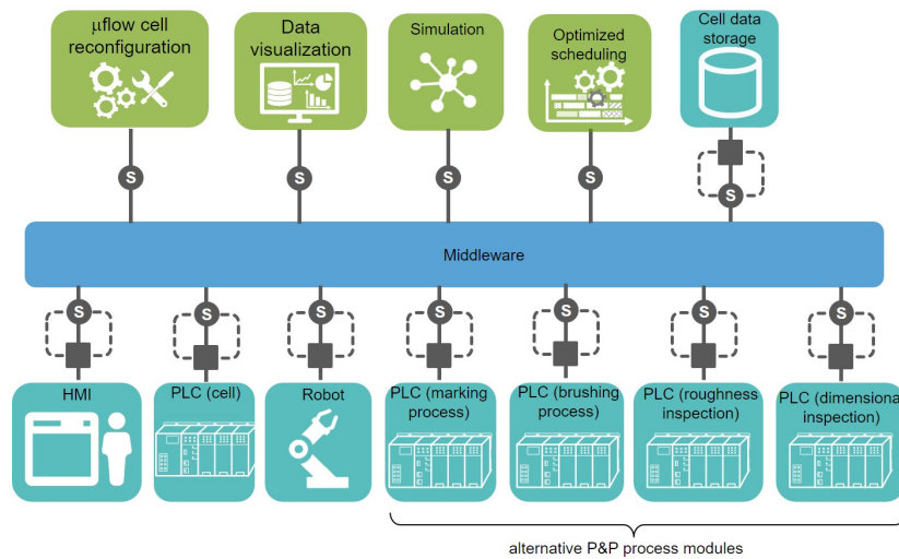
Fig. 5: Architecture Mapping for the GKN Use Case.
