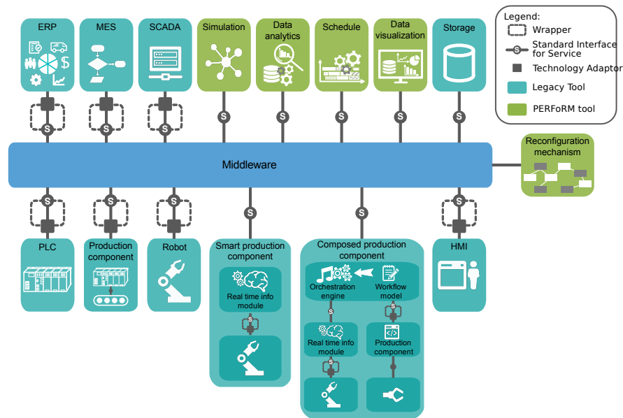
Fig. 1: PERFoRM System Architecture.
