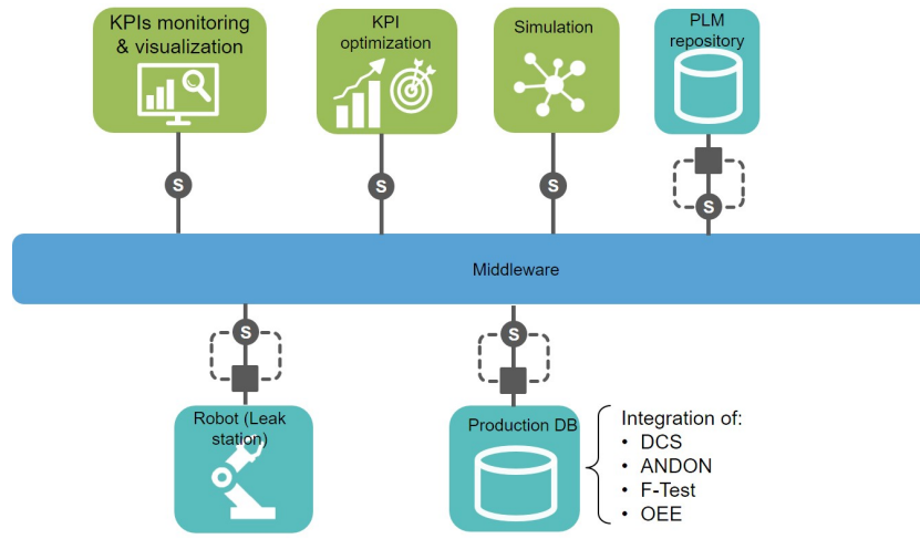
Fig. 4: Architecture Mapping for the Whirlpool Use Case.
